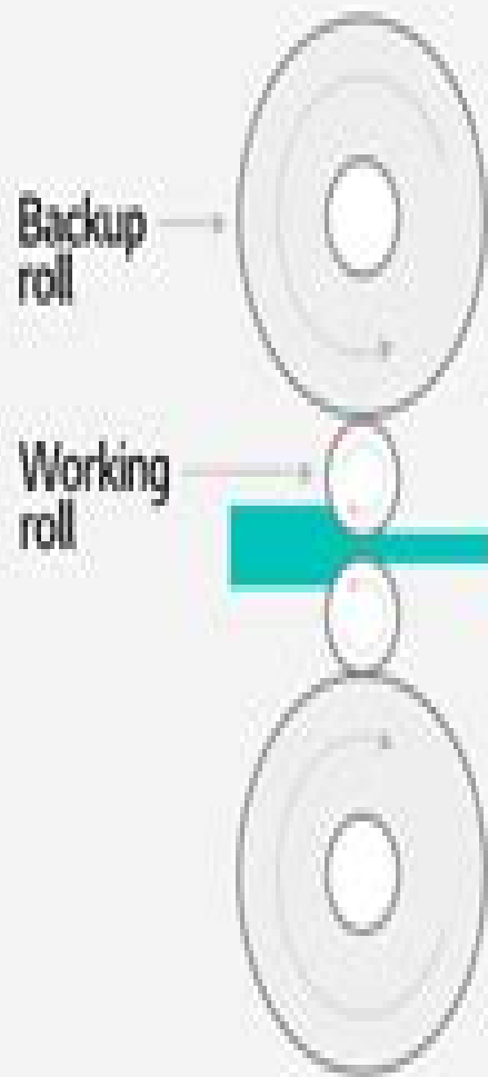
Working rolls and backup rolls in the rolling mill
