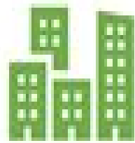
Local environment
