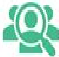
Target object
