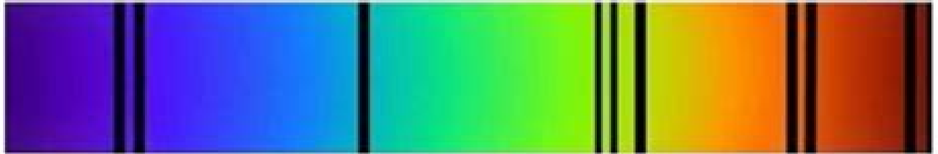
Redshifted spectrum
