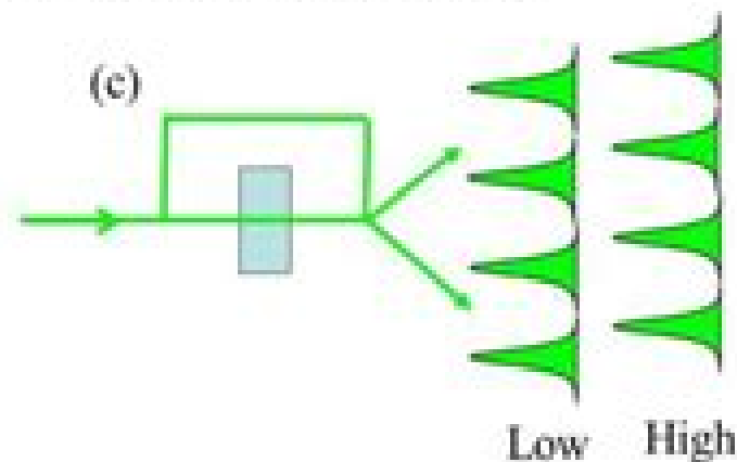
Nonlinear Interferometry
