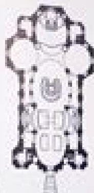
Fig. 11. Section Plan of the Church of Santa Maria della Spina, Florence. (Reproduced from the author's book, "The Architecture of Brunelleschi.")
