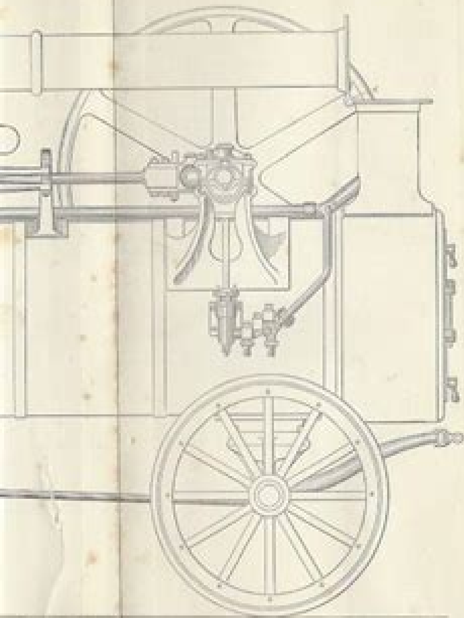
FIG. 2.—Elevation.
