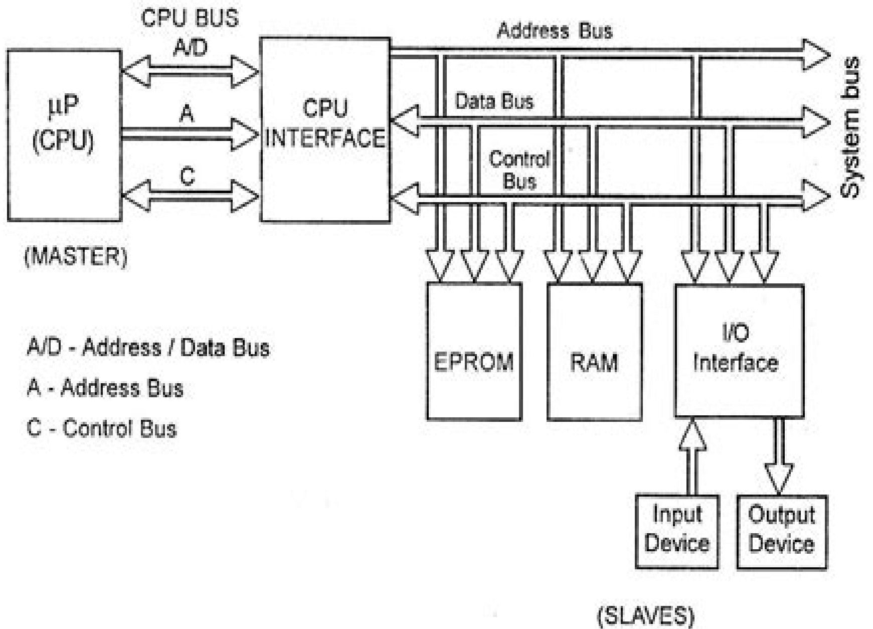
Fig : 1.1 Microprocessor Based System (organisation of microcomputer)
