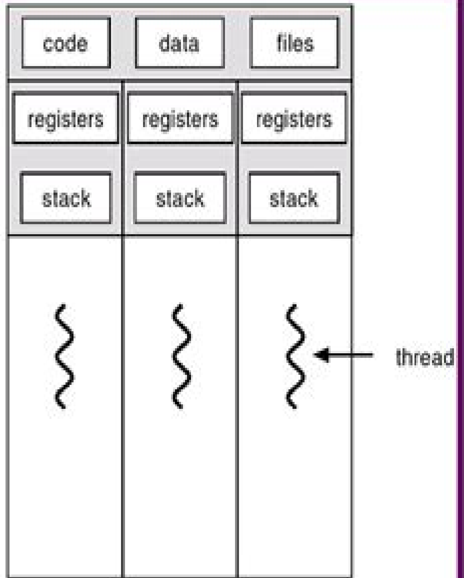
multithreaded
