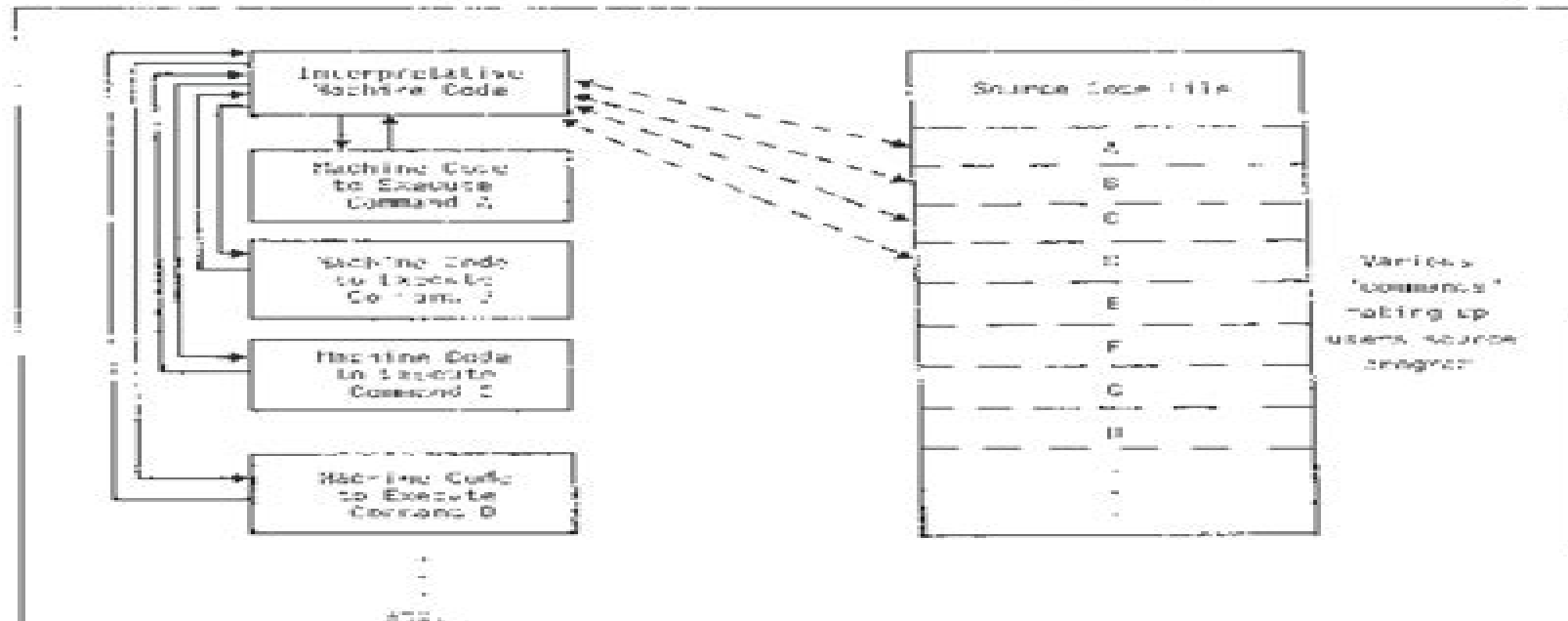
Figure 1. The interpretative cycle of common parts of languages such as BASIC. After assembly, each command in the source file, the interpreter searches for and branches to the corresponding block of machine code; then, program execution always resumes within the interpreter.
