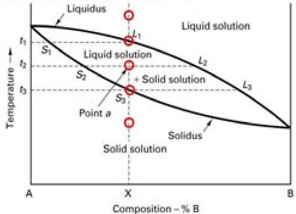
FIGURE 4-8 Equilibrium diagram showing the changes that occur during the cooling of alloy X.
