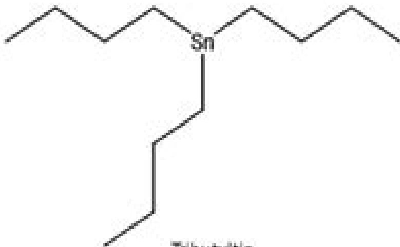
Tributyltin
