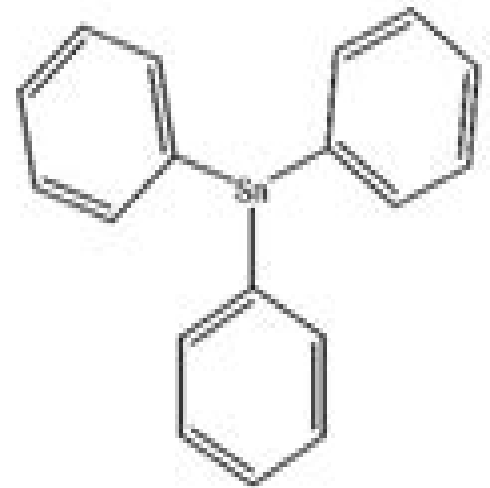
Triphenyltin
