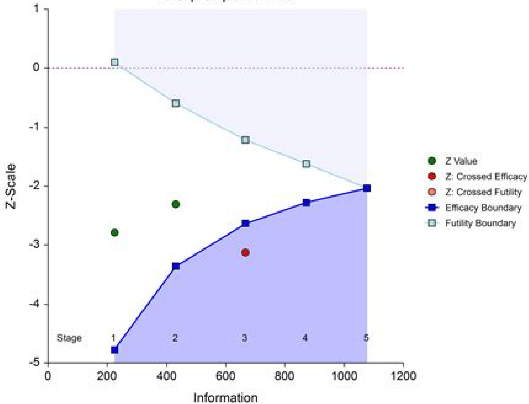
Group-Sequential Plot
