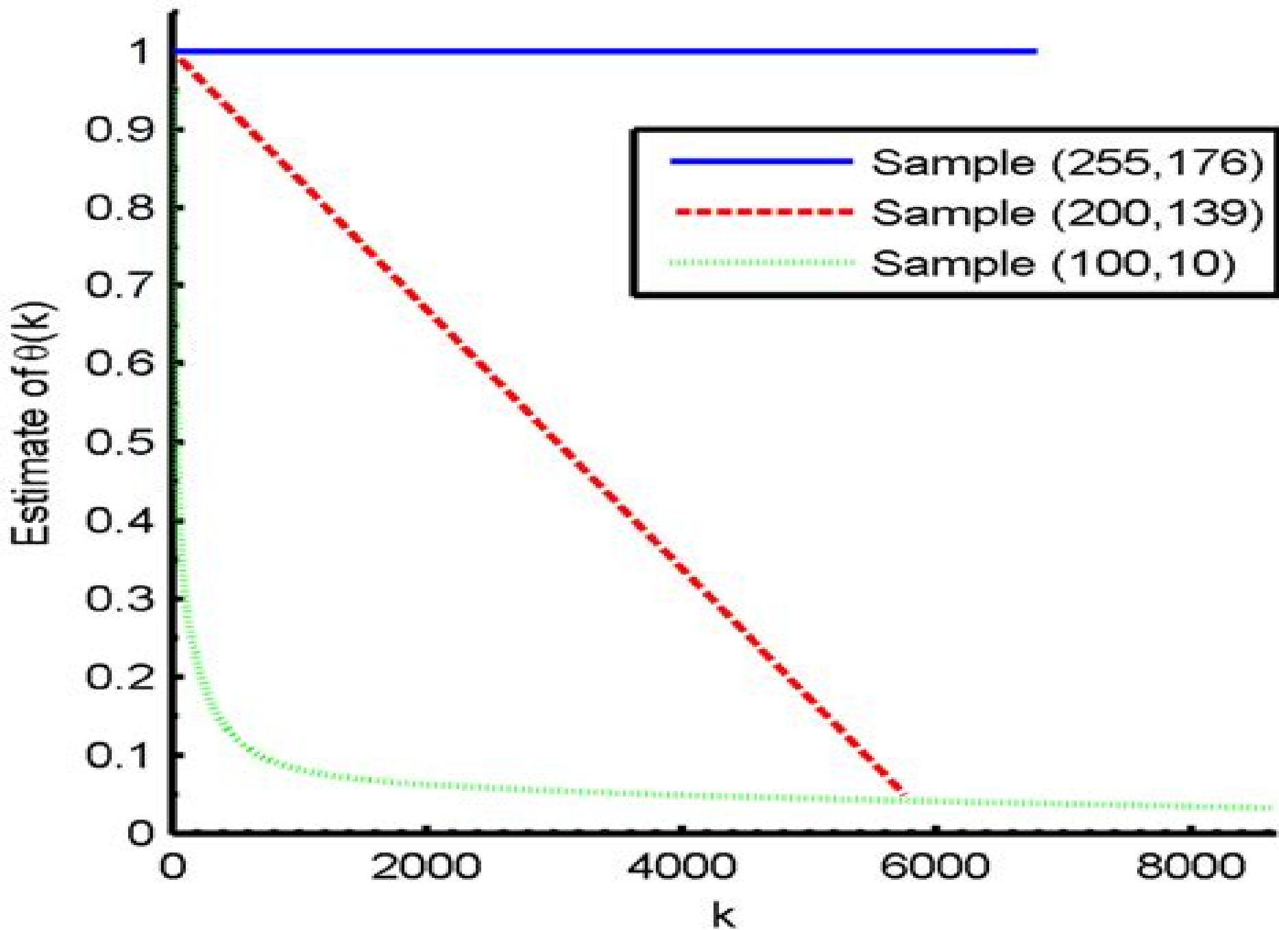
Estimates of \theta(k)
