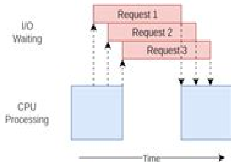
(c) Single-threaded process with asyncio
