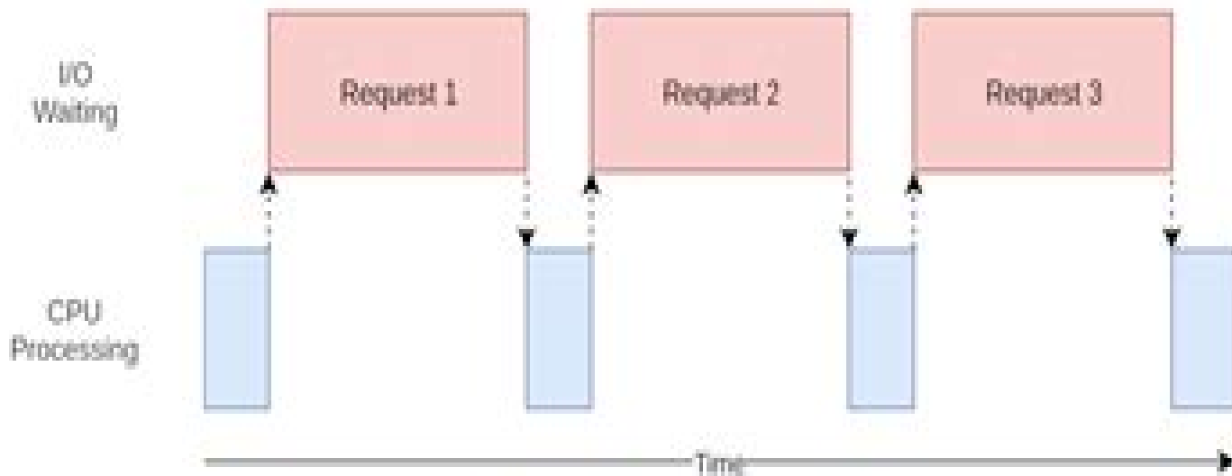
(a) Single-threaded process
