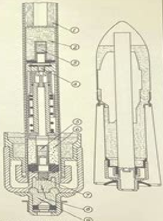
Fuze Assembly & Complete Grenade Scale - 1:100
