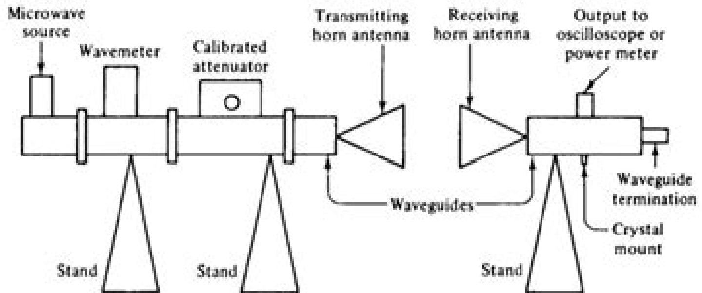
Mr. V. Sudheer Raja Figure 0-1 Microwave system.
