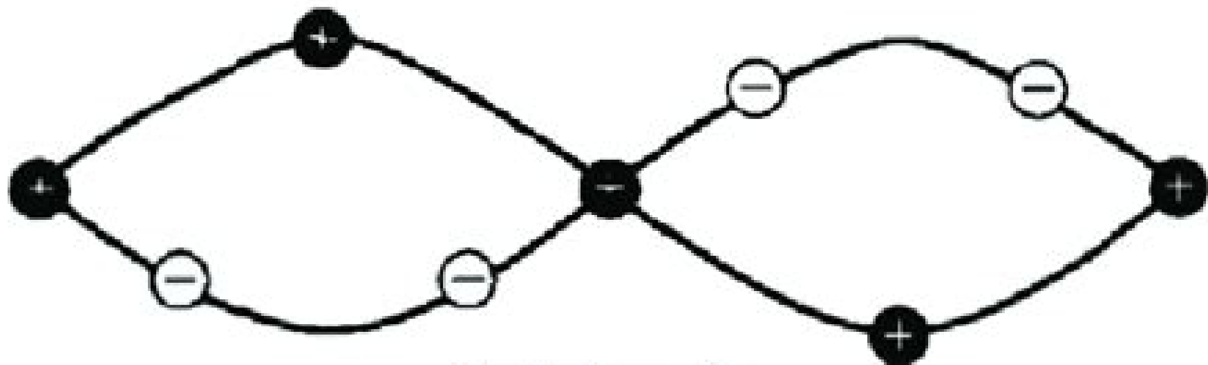
Optical mode
