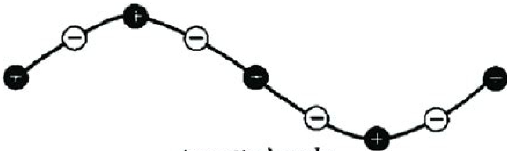
Acoustical mode
