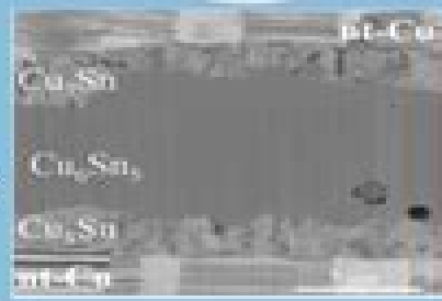
solder after heating
