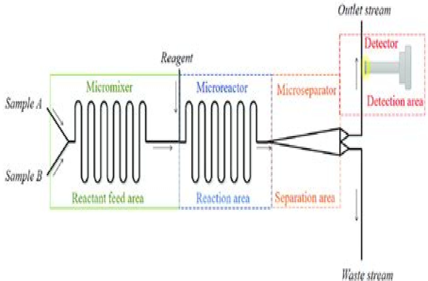
Figure 2. Micro-total analysis system ( \mu TAS) scheme.
