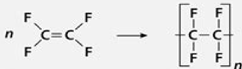
Tetrafluoroethylene
