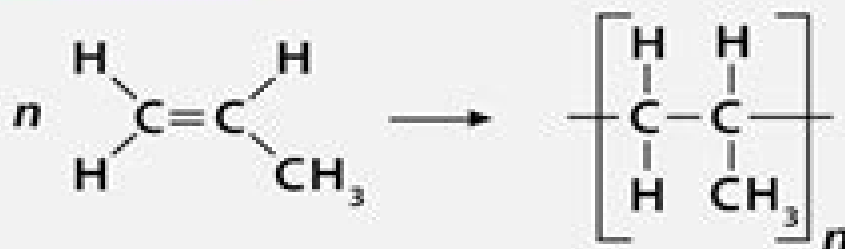
Propene
