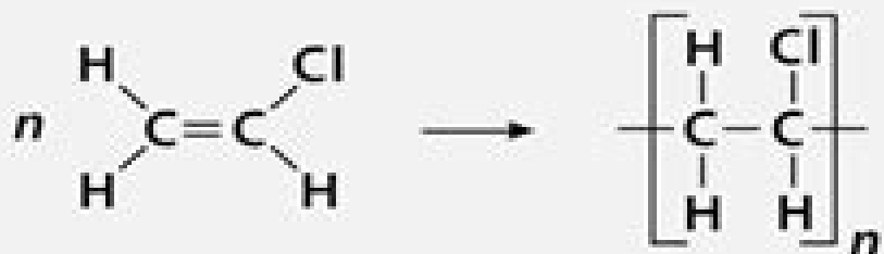
Vinyl chloride
