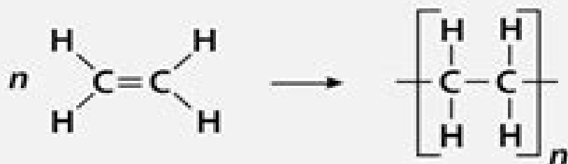
Ethylene
