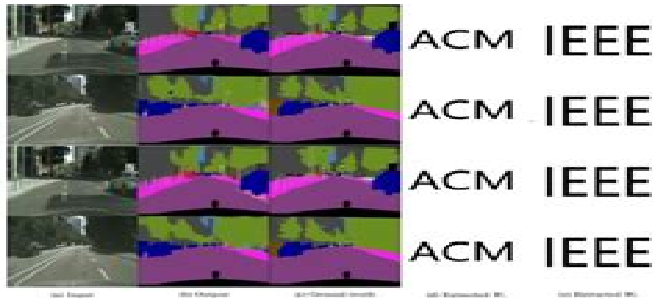
Fig. 3. Visual examples for the marked images and the extracted watermarks. The first two rows correspond to the HVS-RGB framework and the last two rows correspond to the HVS-YUV framework. Notice that, the input in the first row is identical to that in the third row, and the input in the second row is identical to that in the fourth row.
