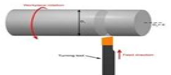
Parting
