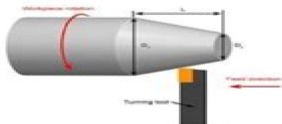
Taper Turning
