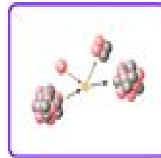
Laws of Nuclear Physics
