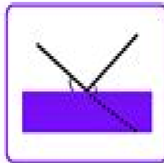
Laws of Solid State Physics
