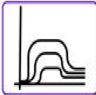
Laws of Quantum Mechanics
