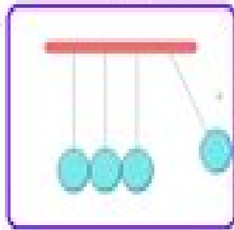
Newton Laws of motion
