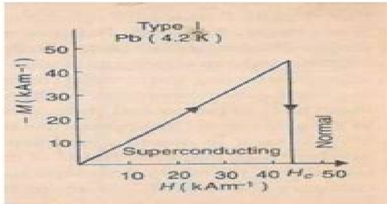
Fig. 4.5. Magnetization curve of pure lead at 4.2 K.
