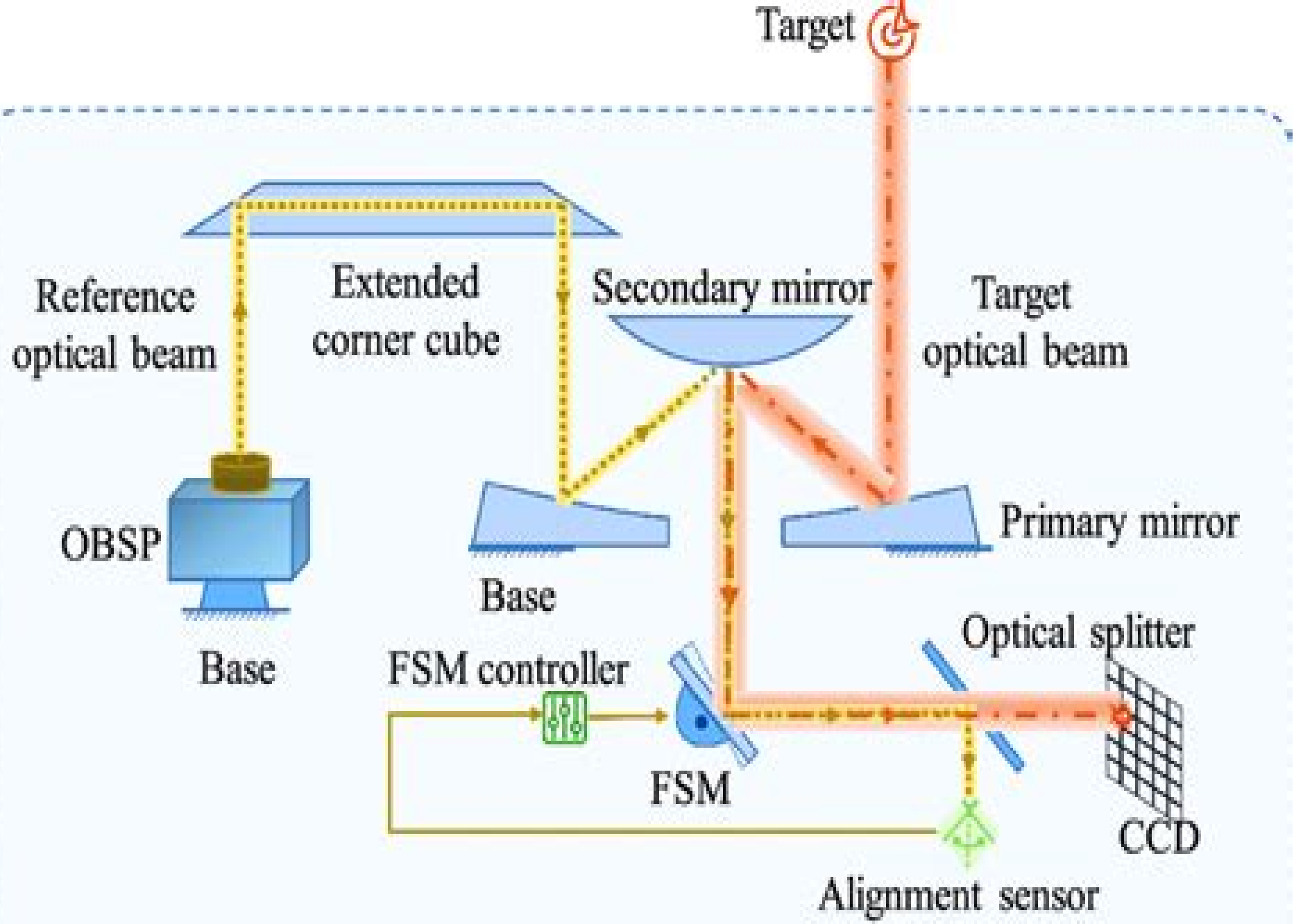
Large-aperture electro-optical system
