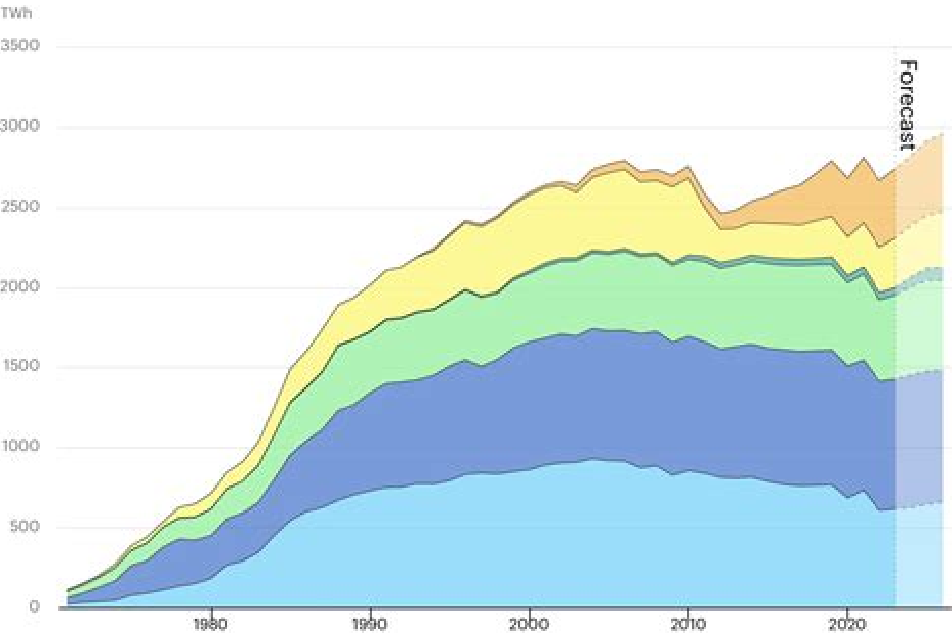
Evolution of nuclear power generation by region, 1972-2026
