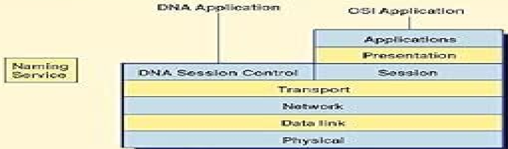
DECnet Phase V Architecture
