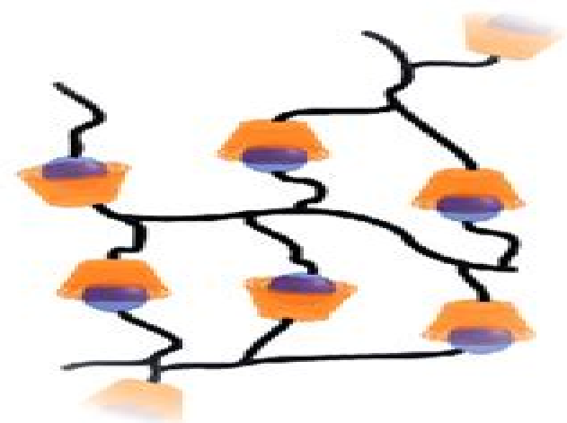
network / gel
