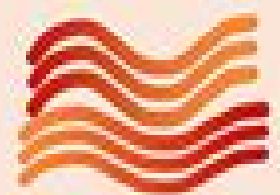
Long-range order
