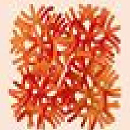
Disordered network
