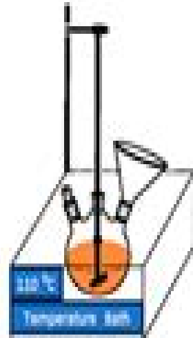
Cellulose dissolution in \text{NMMO}/\text{H}_2\text{O}
