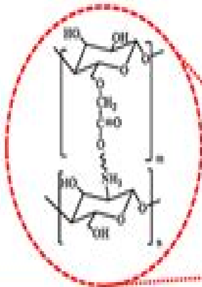
Cellulose dissolution in \text{NMMO}/\text{H}_2\text{O}
