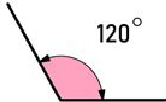
OBTUSE ANGLE greater than 90° less than 180°
