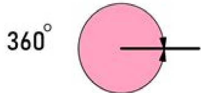
FULL ANGLE exact 360°
