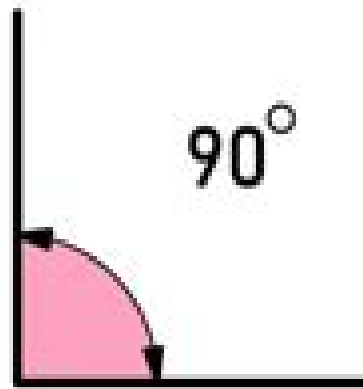
RIGHT ANGLE exact 90°
