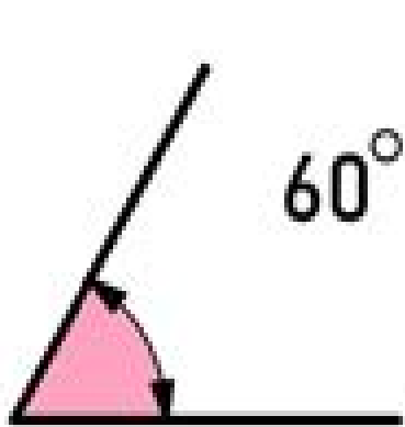
ACUTE ANGLE less than 90°
