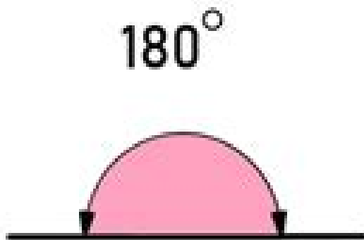
STRAIGHT ANGLE exact 180°
