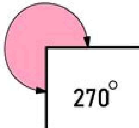
REFLEX ANGLE greater than 180° less than 360°
