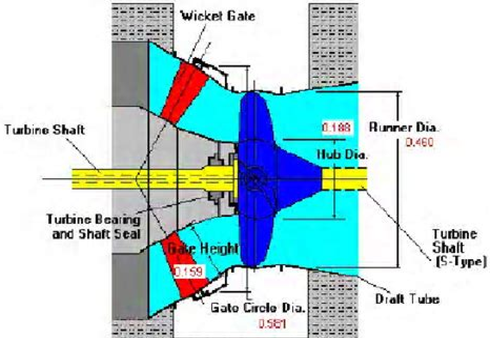
Fig. 2 Runner TURBOPRO design data
