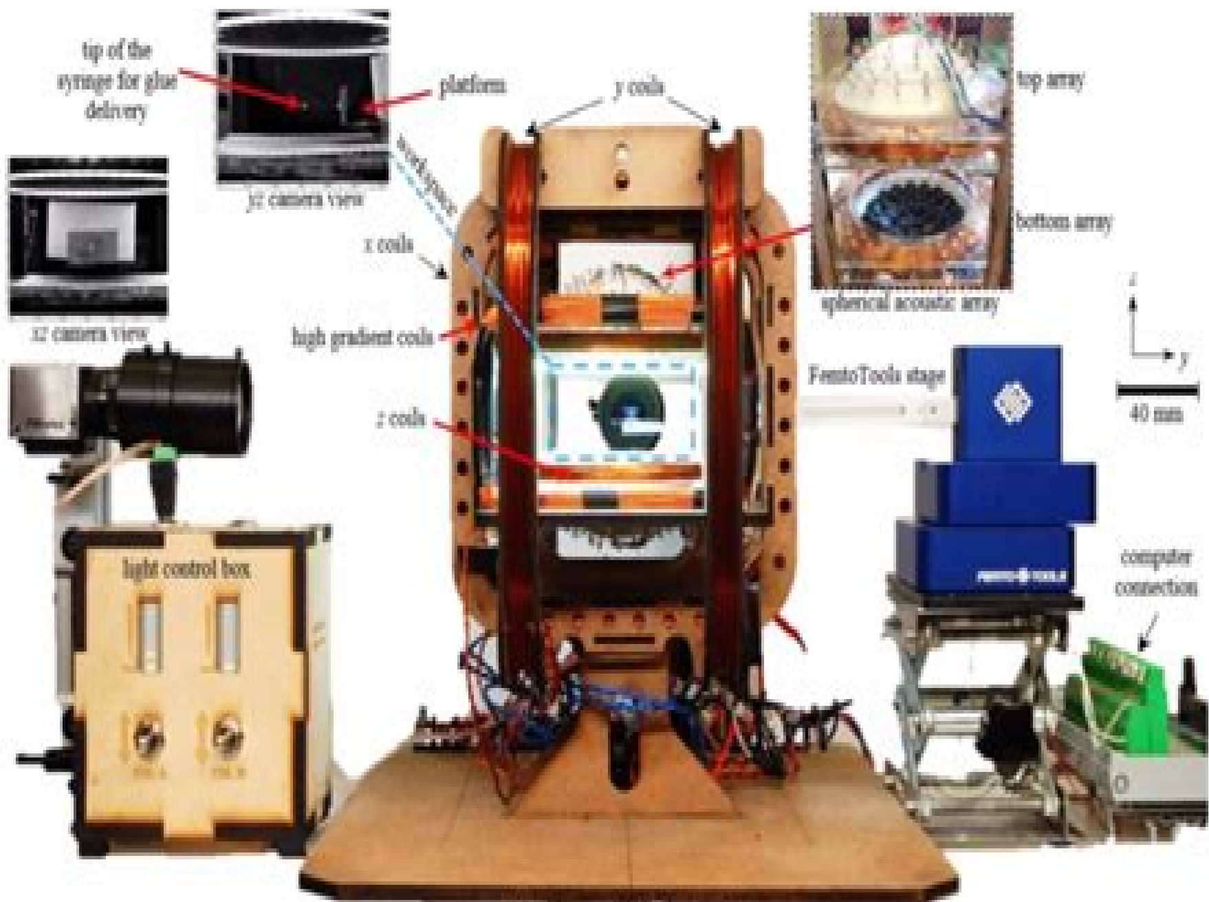
modified square Helmholtz coil system
