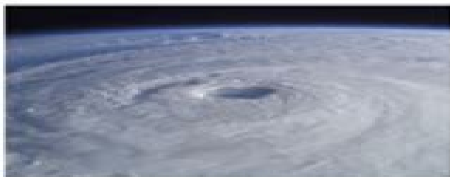
Hurricanes are rotating storm systems.
