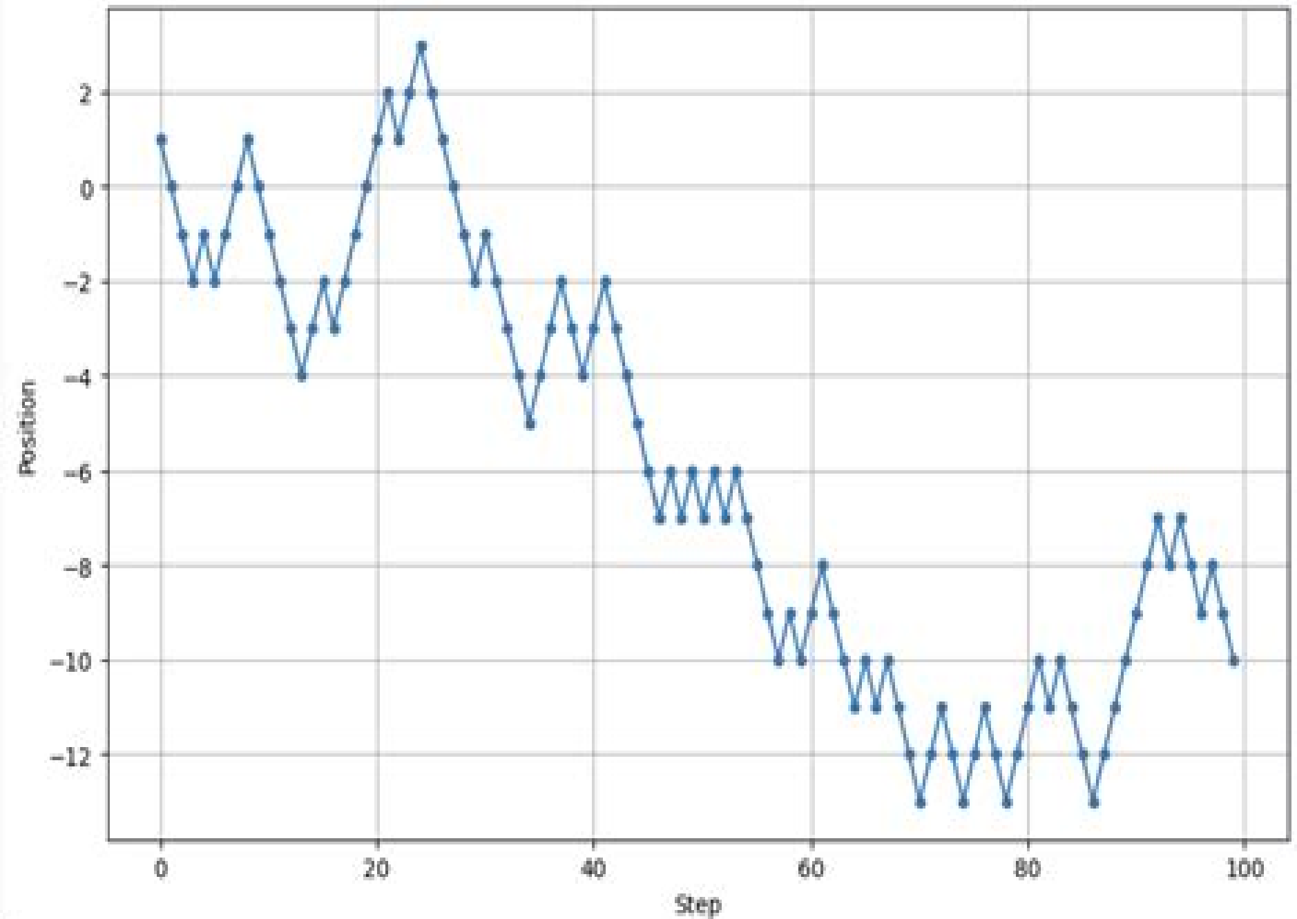
1D Random Walk
