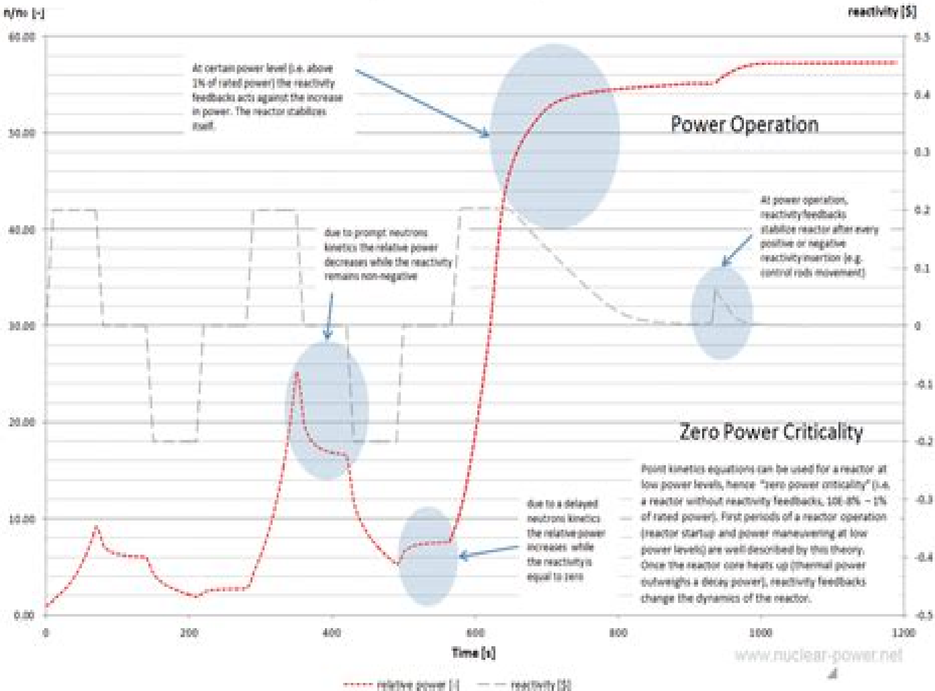
Reactor response after a cyclic symmetric change in reactivity
