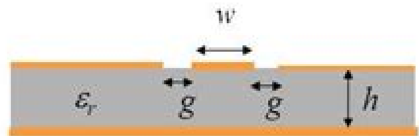
Conductor-backed CPW
