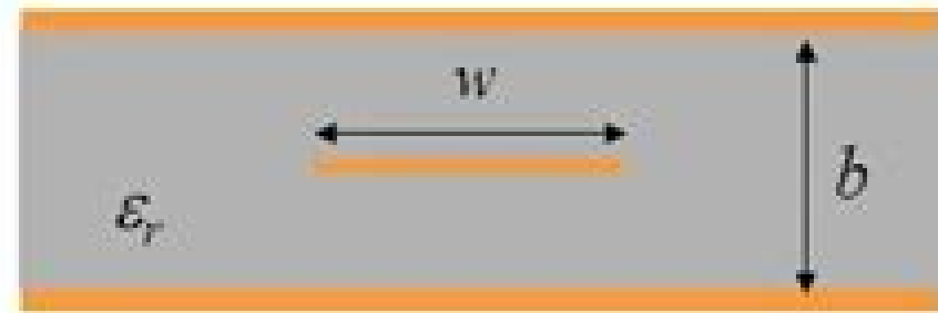
Stripline
