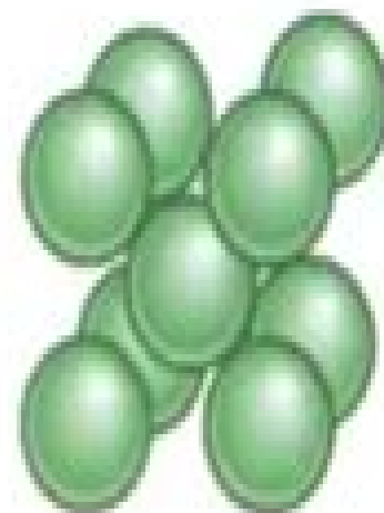
Body-centred Cubic
