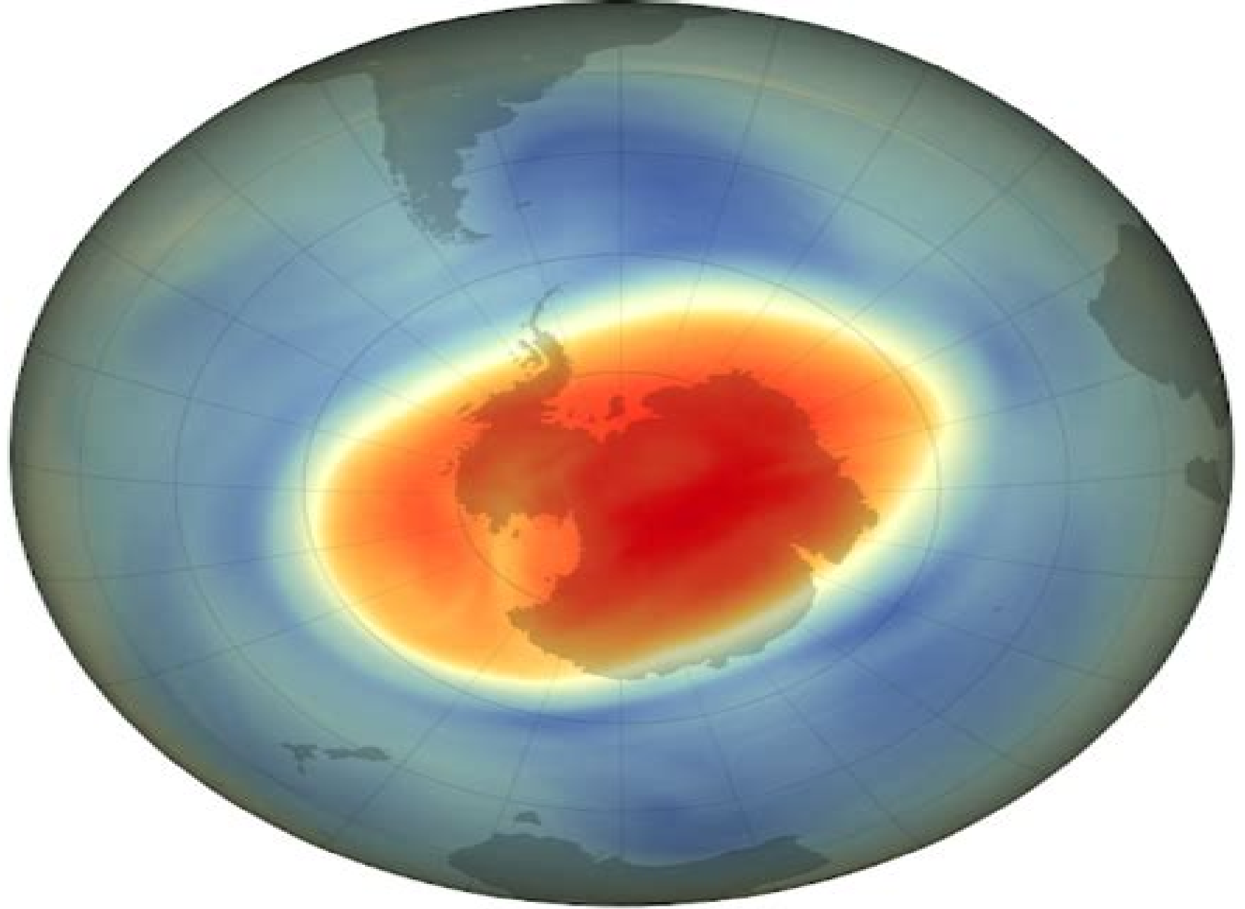
Ozone (Dobson units)
