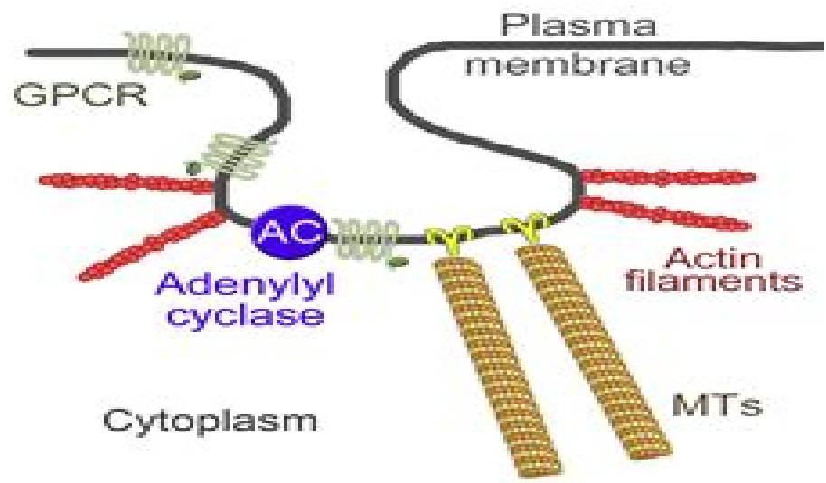
(B) Plasma membrane microdomain formation
