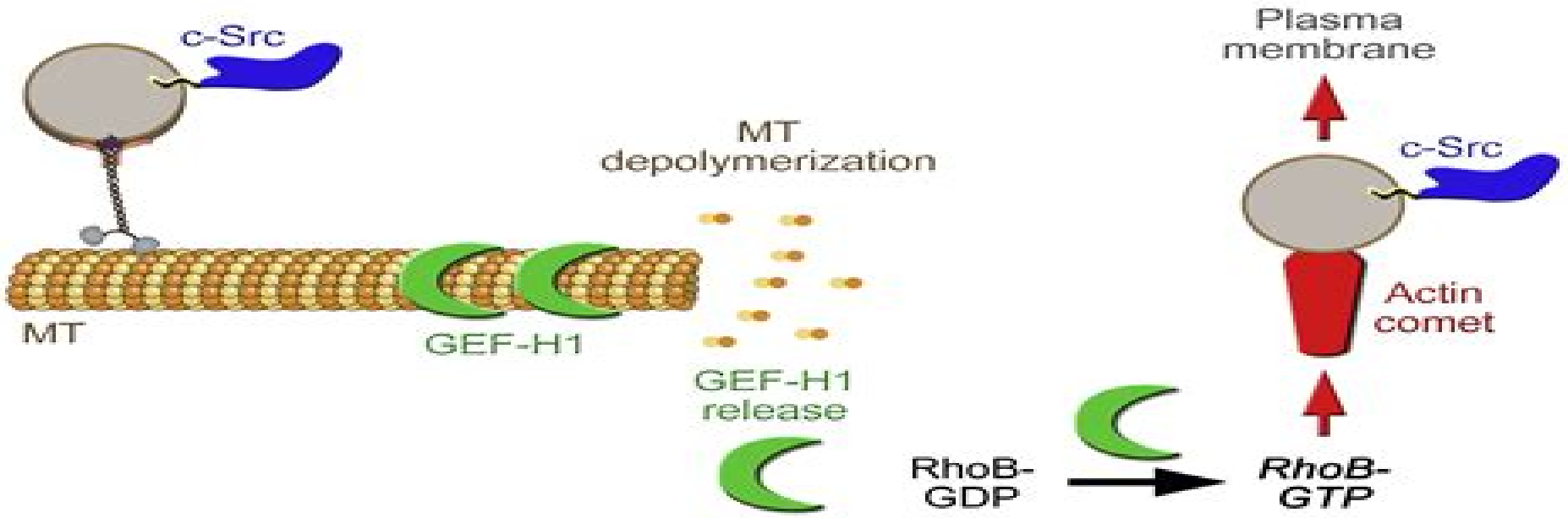
(C) Vesicle trafficking: c-Src delivery to plasma membrane
