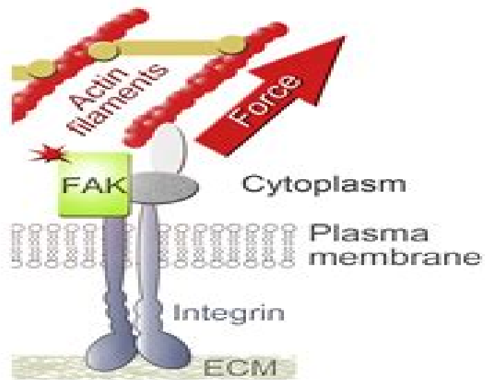
(A) Mechanotransduction: focal adhesions
