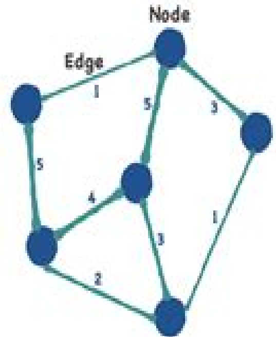
Weighted Graph
