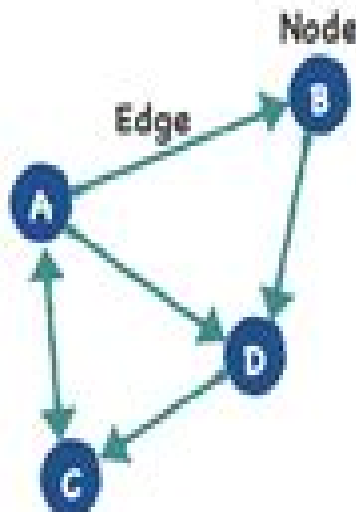
Directed Graph
